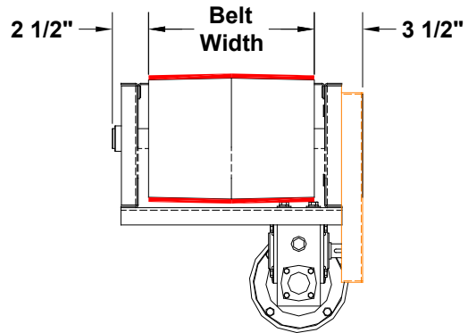
Standard Drive Cross Section
