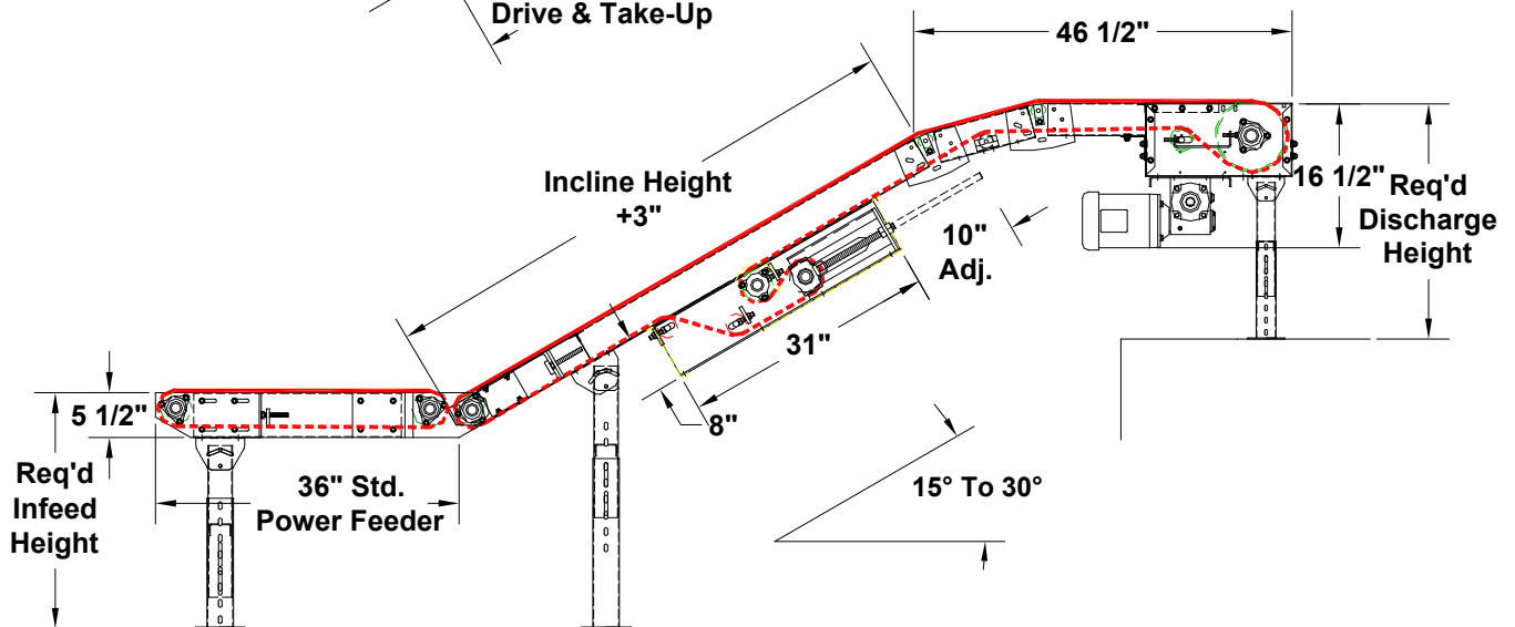
Standard Center Drive & Take-Up
