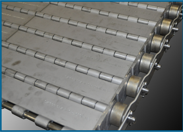
Plain Apron with Radial Sidewings and Outside Sidebars - 2500# Pull
