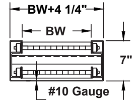
#10 Gauge Bottom Pan Section B-B Intermediate Cross Section
