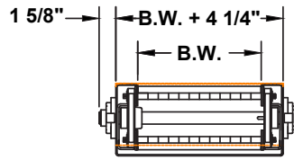
Section A-A Infed with Optional 3-Bolt Flange Bearings
