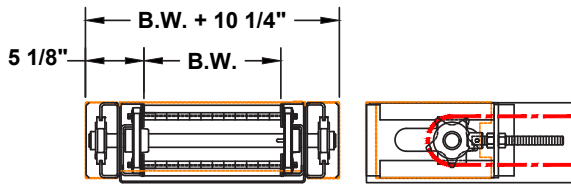
Section A-A Infed with T-Slot Take-Up Bearings
