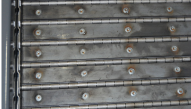
Impact Plates
