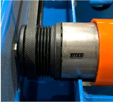
Poly V-Belt Driven Roller
